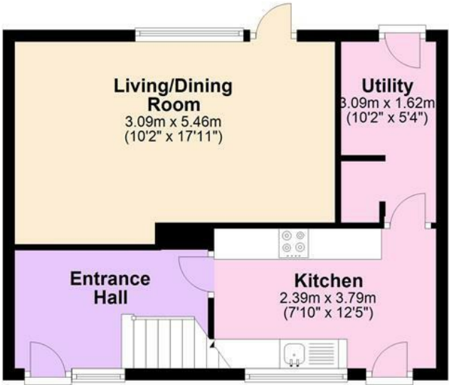
Ground Floor Approx. 40.1 sq. metres (431.3 sq. feet)
